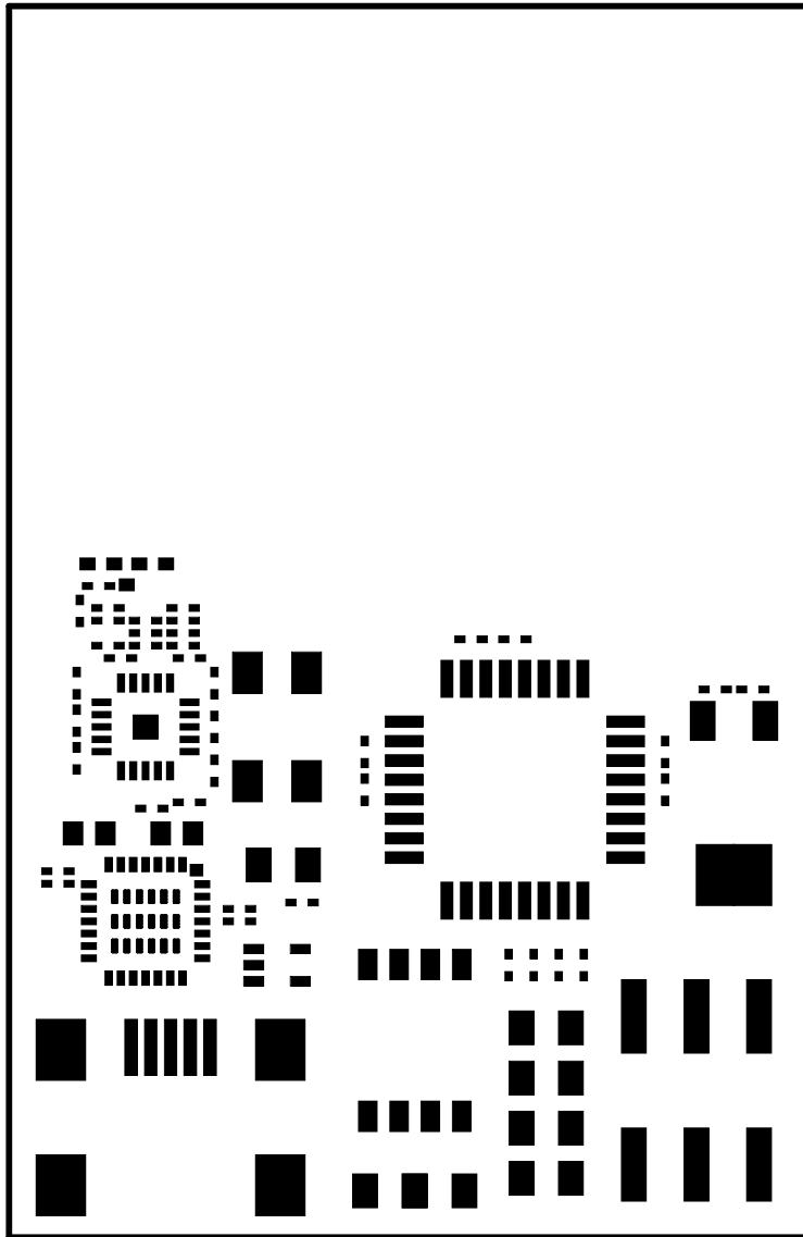
Paste Mask Top
