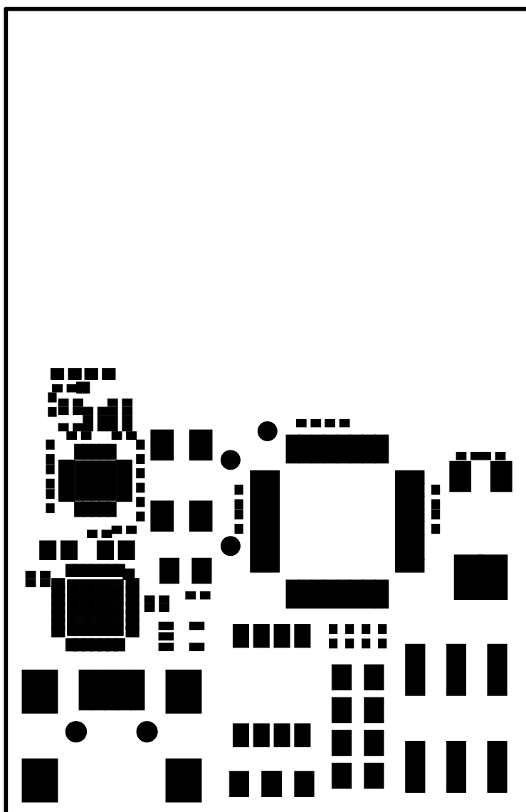
Solder Mask Top
