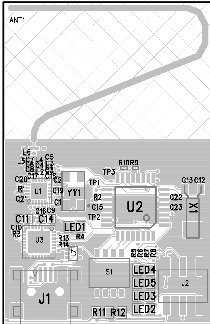
Top Assembly Drawing Top
