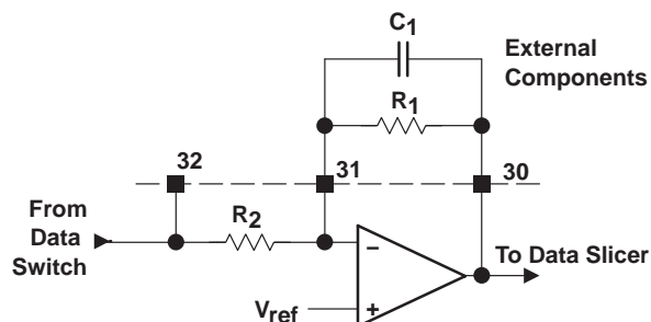
Figure 11. 1 st -Order Low-Pass Filter Example
