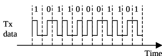
Figure 12. Manchester encoding
