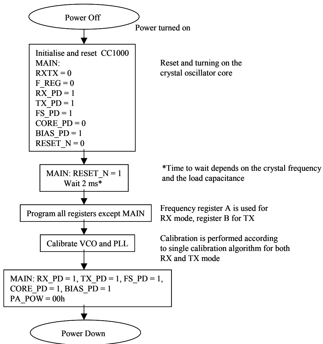
Figure 18. Initializing sequence
