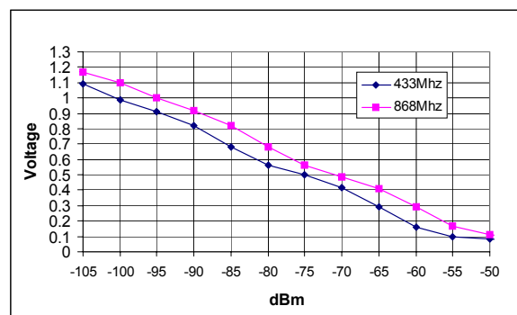
Figure 22. RSSI voltage vs. input power
