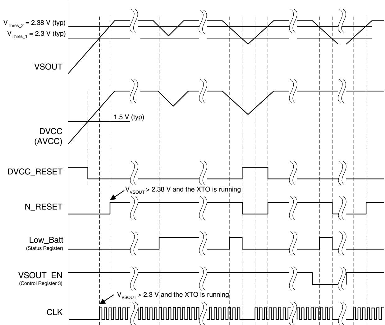
Figure 5-3. Reset Timing
