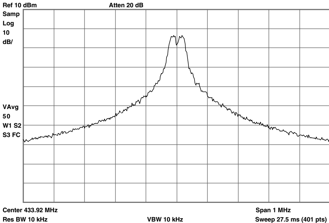
Figure 3-9. FSK-modulated TX Spectrum (433.92 MHz/20 kBaud/ \pm 16.17 kHz/Manchester Code)
