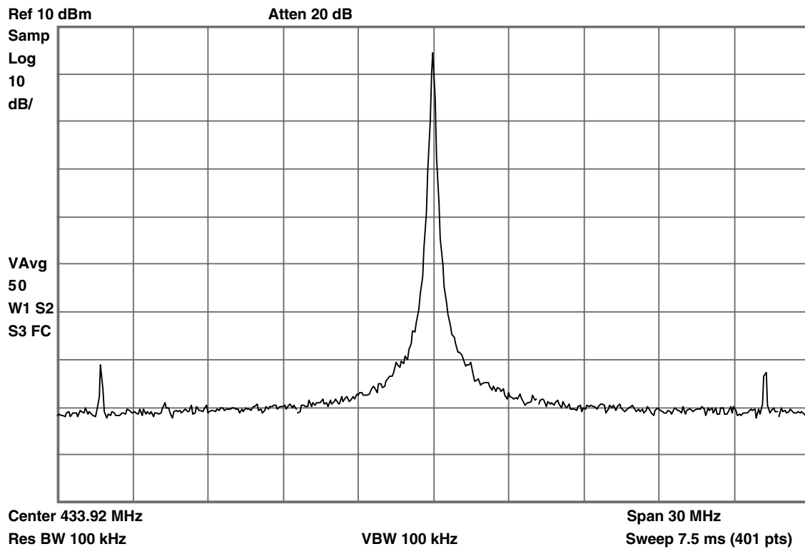
Figure 3-7. FSK-modulated TX Spectrum (433.92MHz/20 kBaud/ \pm 16.17 kHz/Manchester Code)
