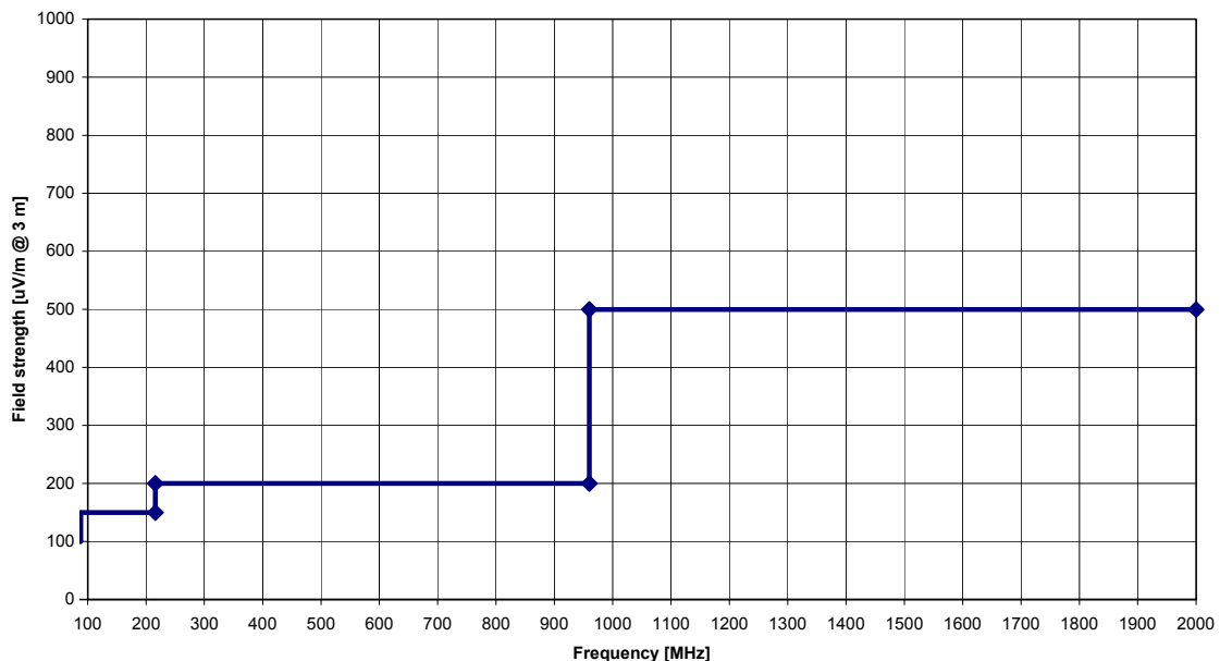
Spurious emission requirement (15.209)
